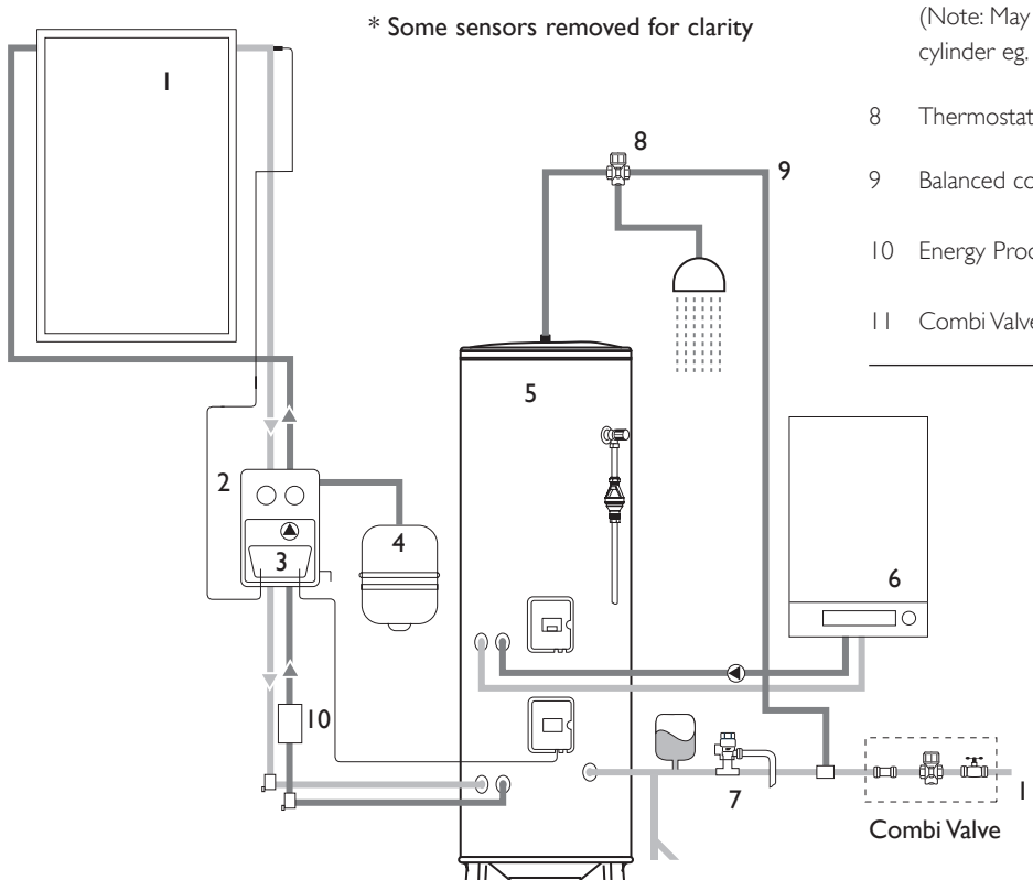
Fig. 1 Unvented System Example
